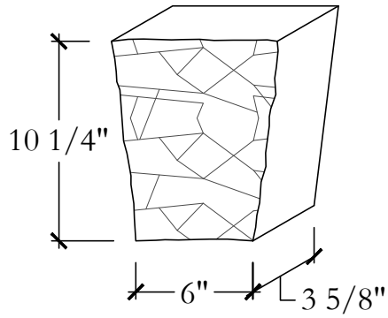
ISOMETRIC
